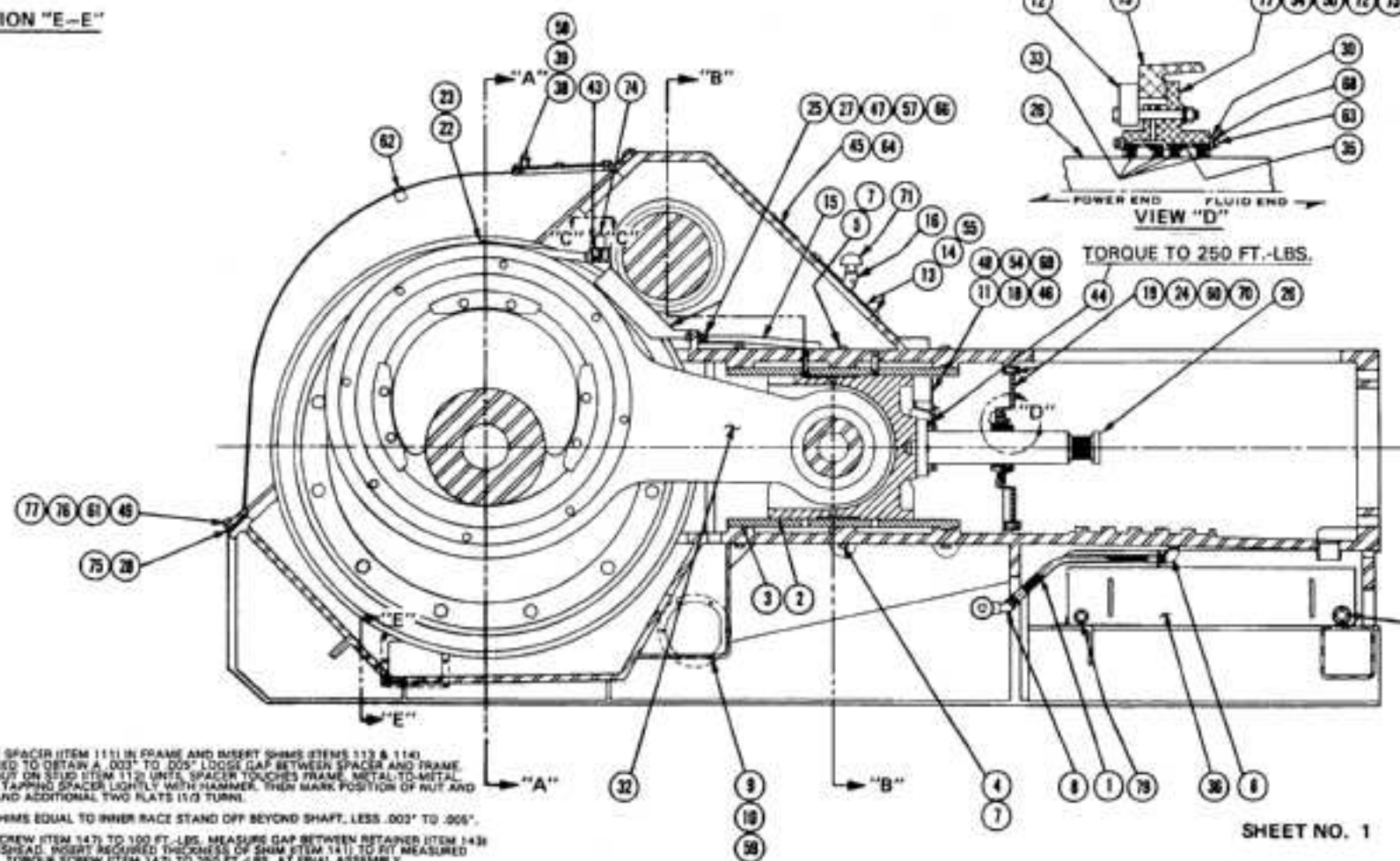
SECTION "E-E"
