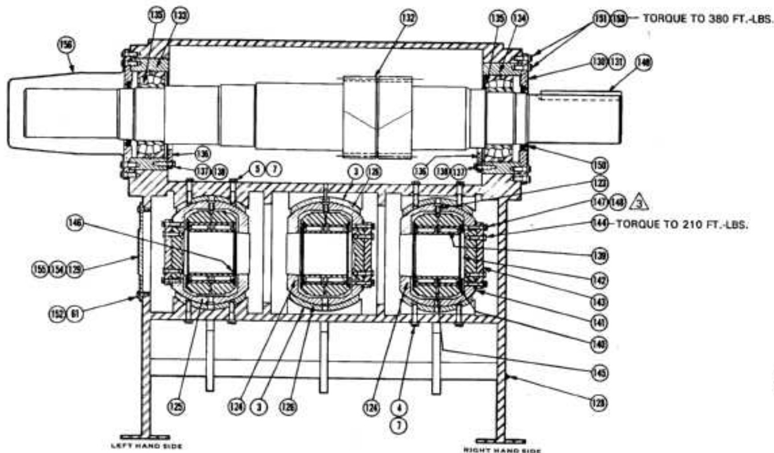
SECTION "B-B"
